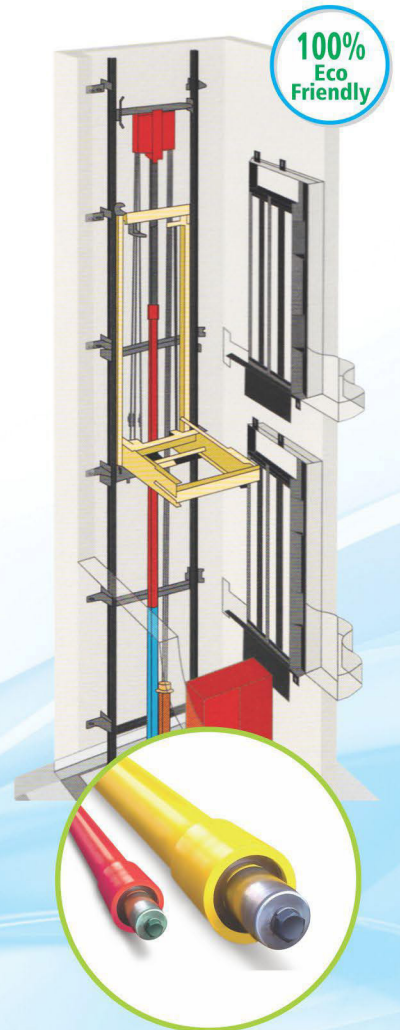
Hydraulic Cylinder
